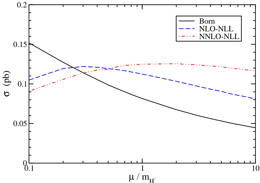
Figure 5: The scale dependence for production of a charged Higgs with mass m_{H^-} = 500 GeV at the LHC.
